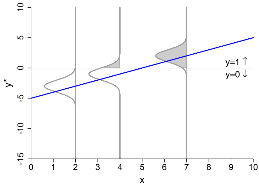
Figure 1: The link between y^* = \beta_0 + \beta_1 x + \varepsilon and \Pr(y=1 | x) with \text{Var}(\varepsilon) = \sigma^2 .
