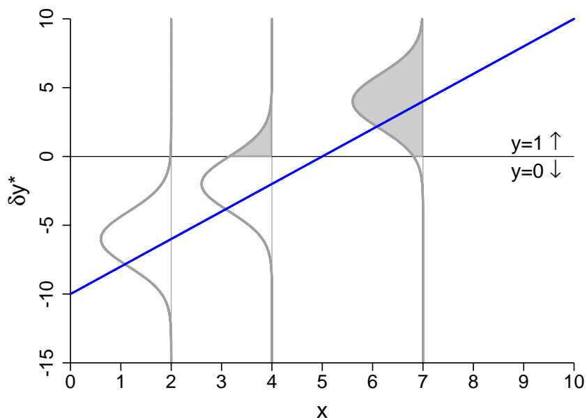
Figure 2: The link between \delta y^* = (\delta\beta_0) + (\delta\beta_1)x + \delta\varepsilon and \Pr(y=1 | x) with \text{Var}(\delta\varepsilon) = \delta^2\sigma^2 .
