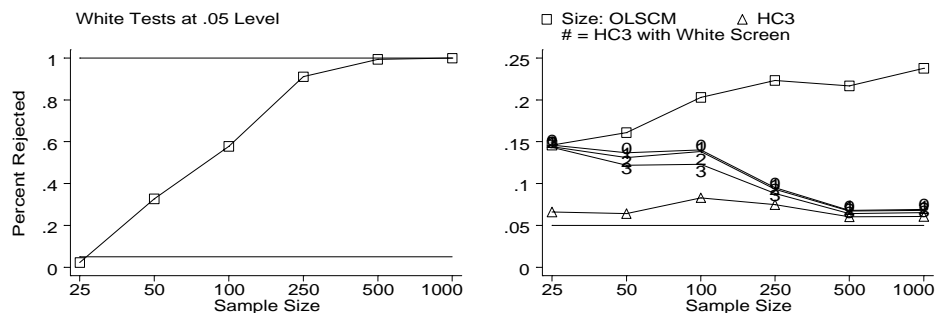
Figure 4: Power of the White test for heteroscedasticity at the .05 level and size of t -tests of \beta_3 after screening with a White test. Errors are \chi_5^2 with heteroscedasticity associated with x_3 and x_4 .
